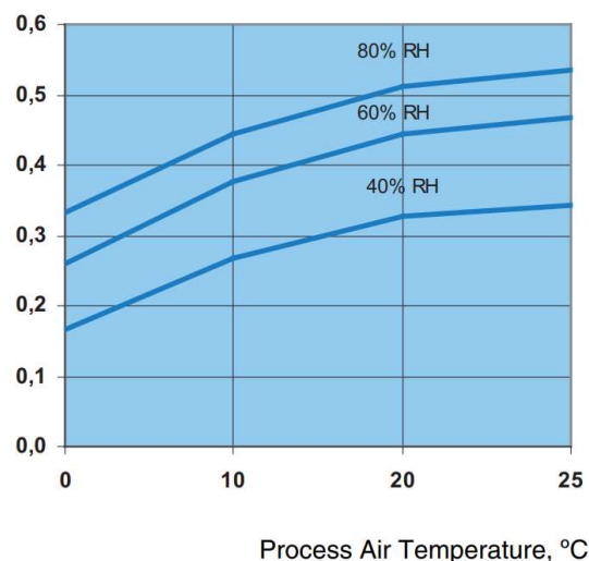
Dehumidification capacity
